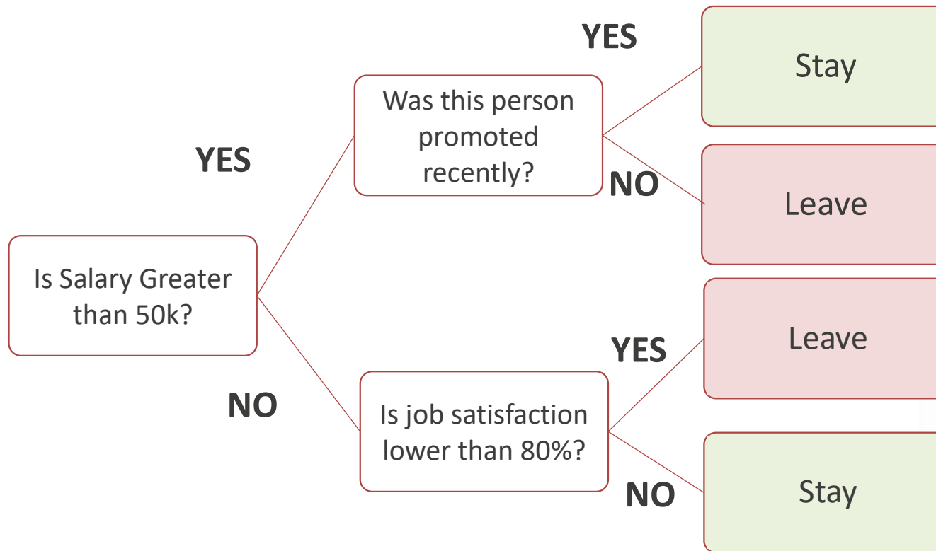
An example decision tree
